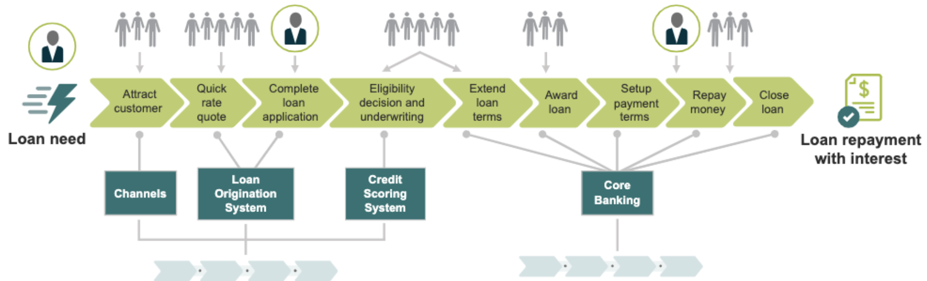
Figure 3. Fulfillment DVS pattern for a consumer loan
